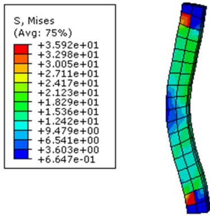
Fig 13. The results for model 4 (without tensile tendon–200kN load).
